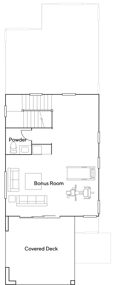
Third Floor
