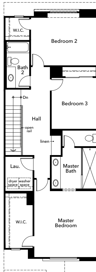
Second Floor
